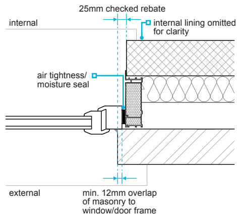
Figure 4: Checked rebate
