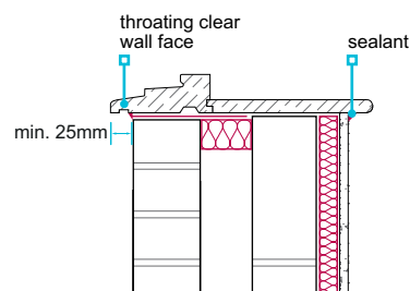
Figure 2: Throating to window sill — cavity masonry wall
