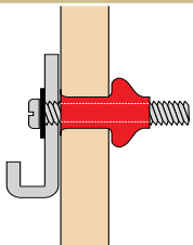
Expanding plug
