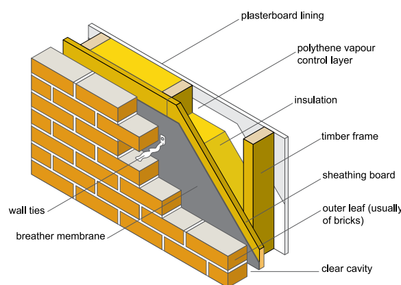
Timber frame external wall construction
