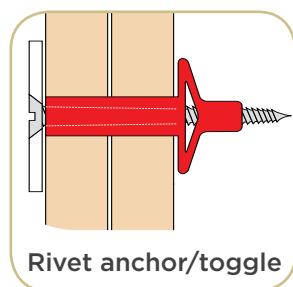
Steel cavity fixing
