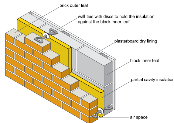
Cavity partially filled with insulation
