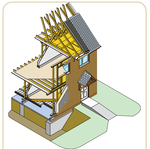
Typical timber frame construction
