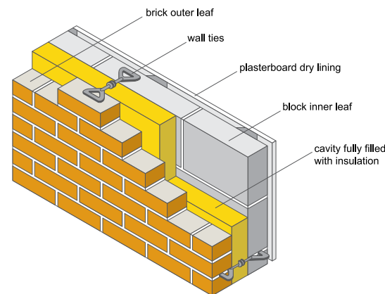
Cavity fully filled with insulation
