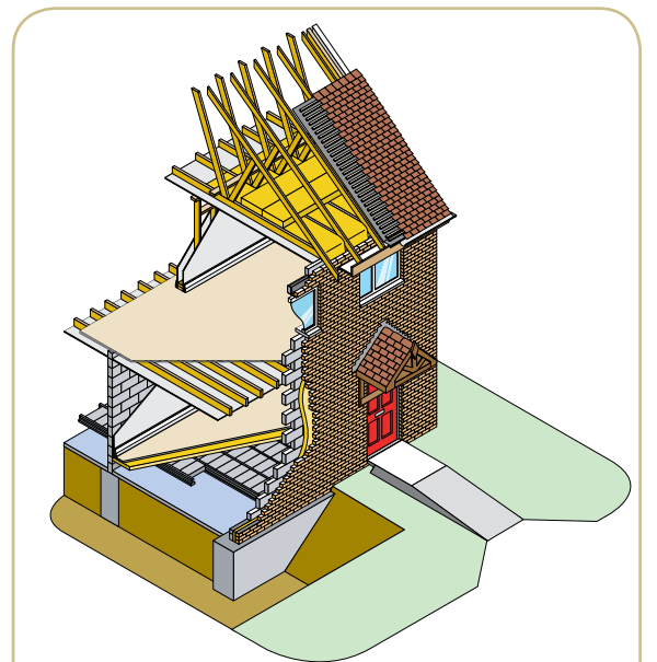
Typical masonry cavity construction
